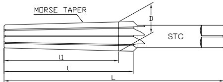
GOST 11182 STRAIGHT SHANK
