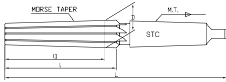
GOST10079 MORSE TAPER SHANK
