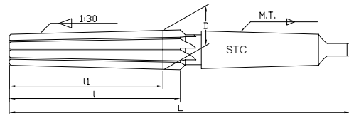
GOST 10082 MORSE TAPER SHANK
