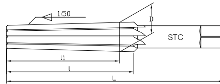
GOST11177 STRAIGHT SHANK
